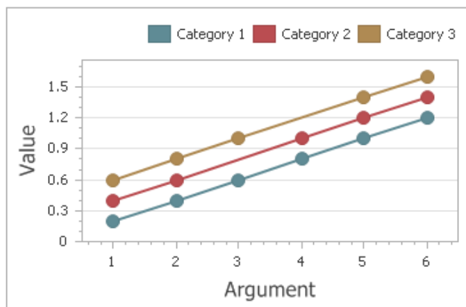
IgnoreEmptyPoints == true
