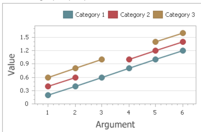
IgnoreEmptyPoints == false
